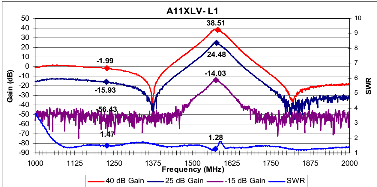
Figure 2. A11XLV L1 Filtered Frequency Response
